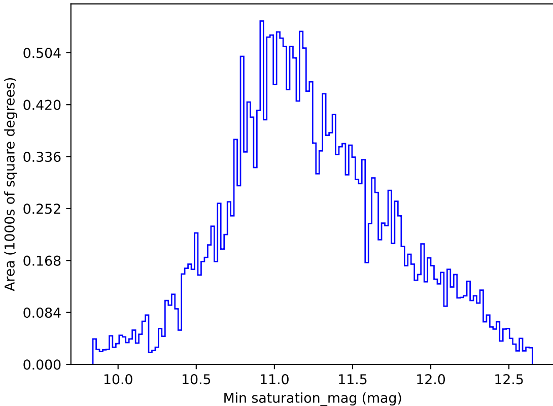
baseline_v3.2_10yrs All sky all bands: Min saturation_mag
