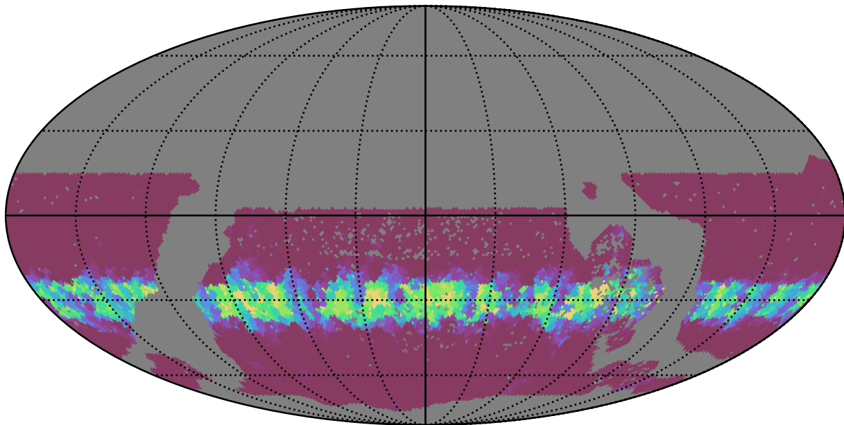
baseline_v3.2_10yrs WFD u band: Min normairmass
