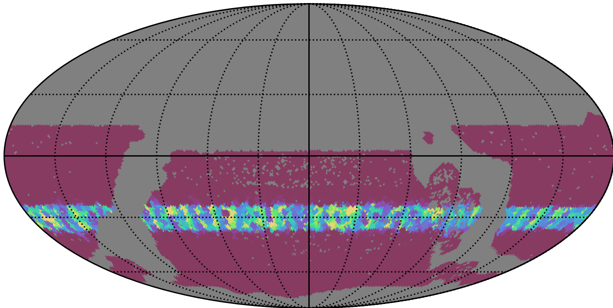
baseline_v3.2_10yrs WFD r band: Min normairmass
