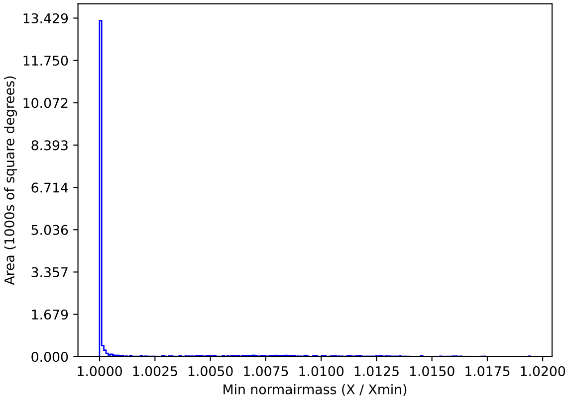
baseline_v3.2_10yrs WFD r band: Min normairmass
