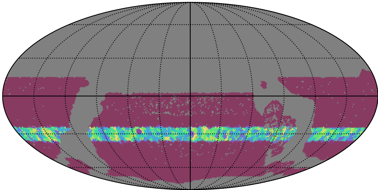
baseline_v3.2_10yrs WFD all bands: Min normairmass
