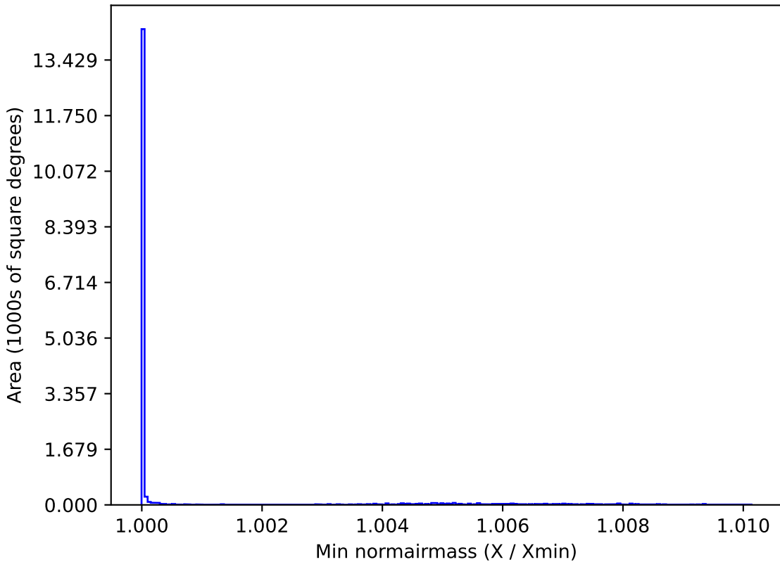
baseline_v3.2_10yrs WFD all bands: Min normairmass
