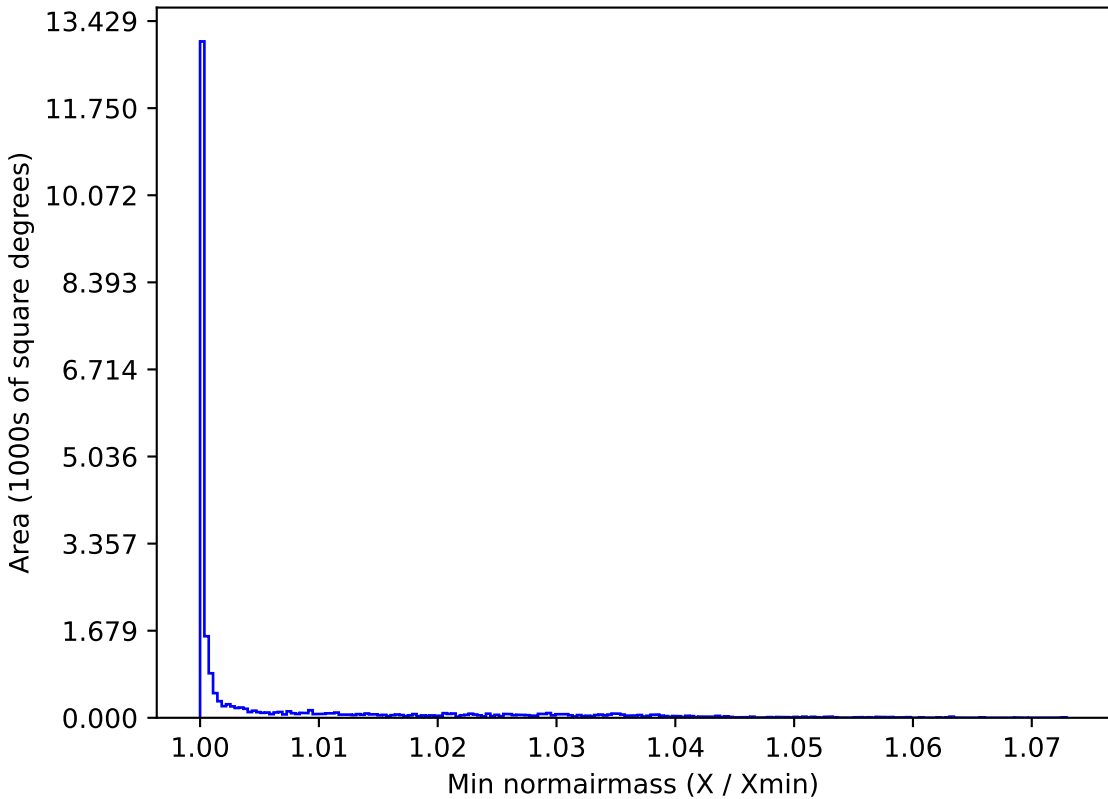
baseline_v3.2_10yrs All sky u band: Min normairmass
