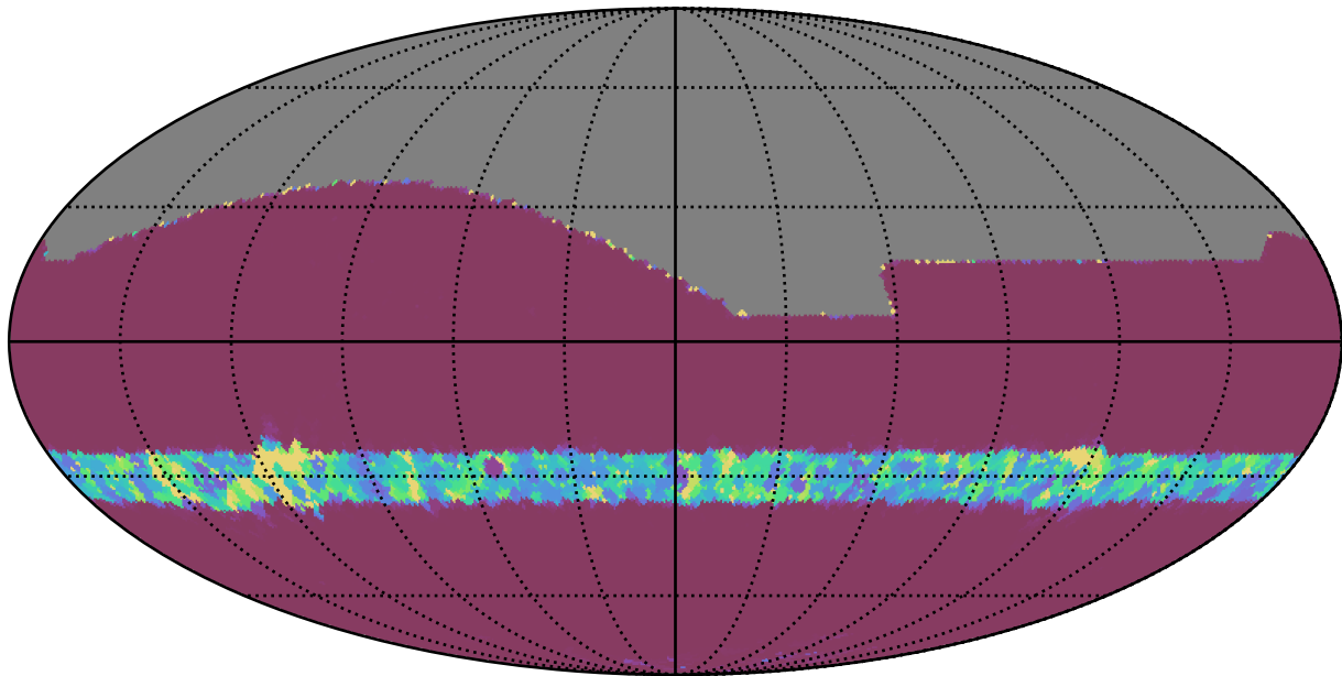
baseline_v3.2_10yrs All sky all bands: Min normairmass
