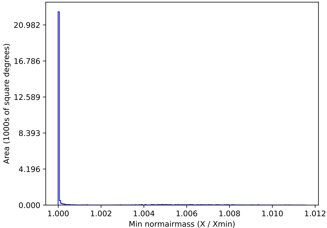
baseline_v3.2_10yrs All sky all bands: Min normairmass
