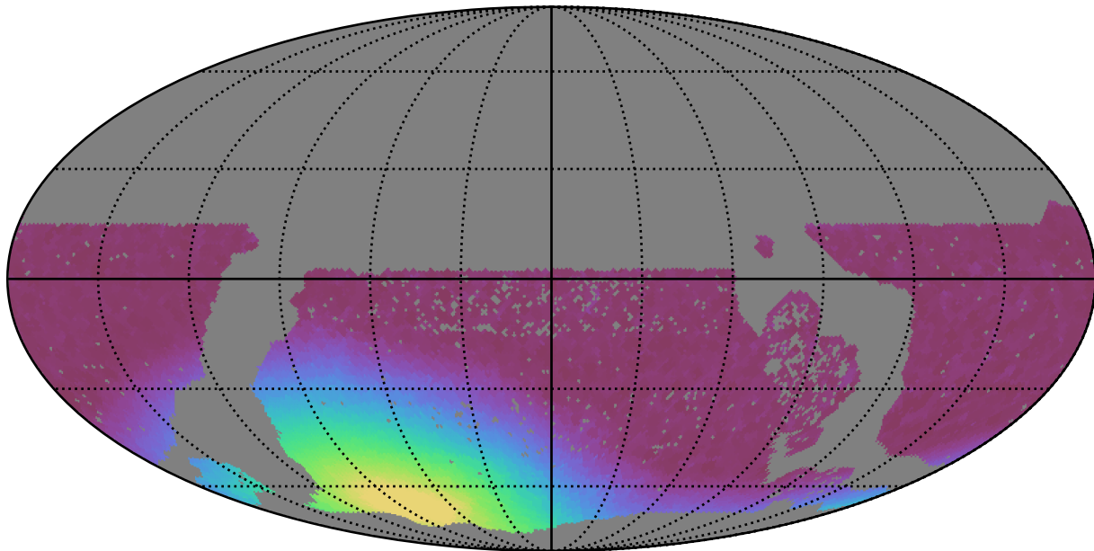
baseline_v3.2_10yrs WFD z band: Min moonDistance
