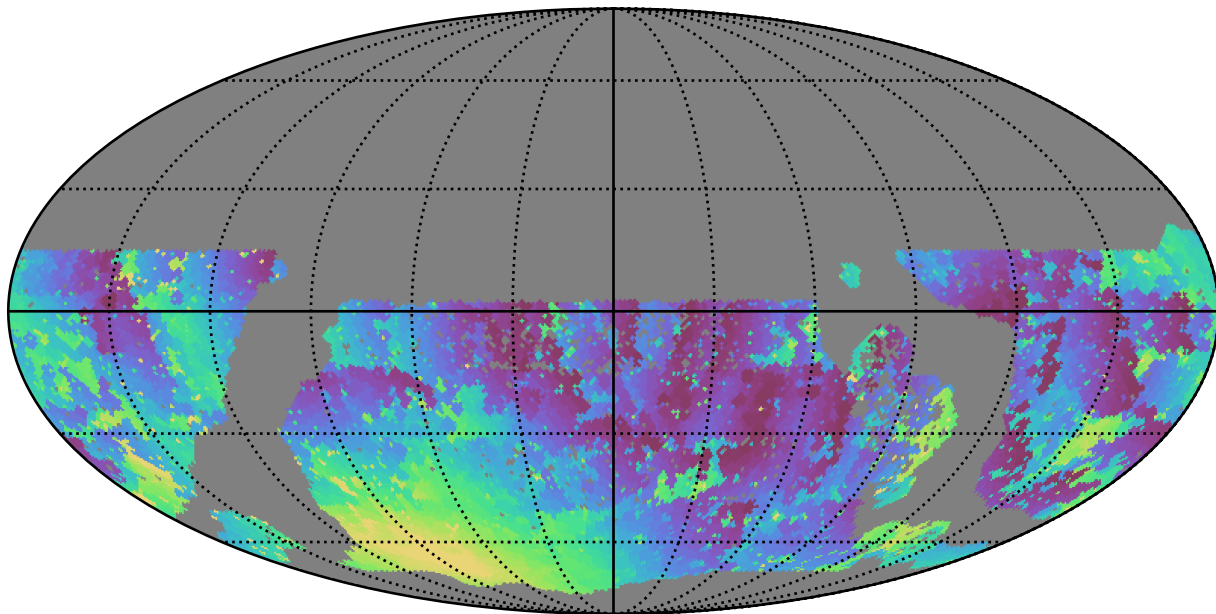
baseline_v3.2_10yrs WFD u band: Min moonDistance
