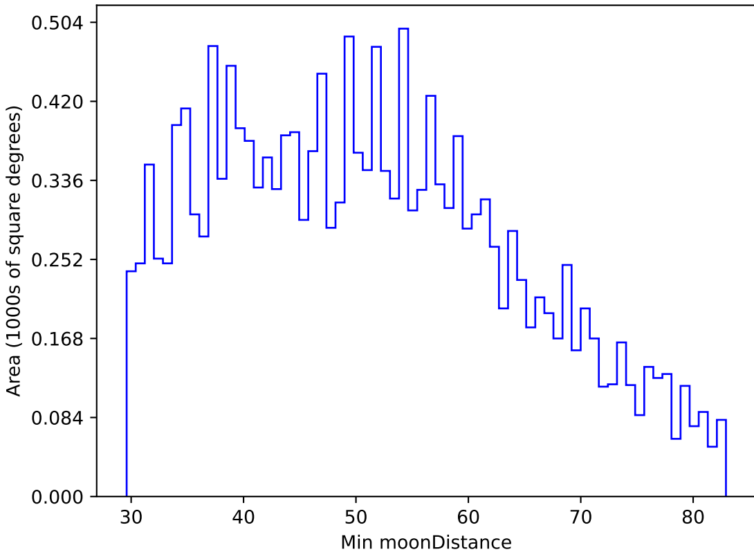
baseline_v3.2_10yrs WFD u band: Min moonDistance
