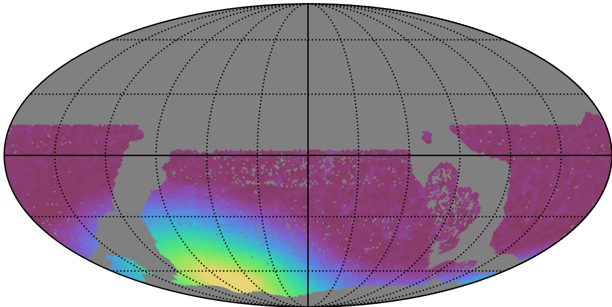
baseline_v3.2_10yrs WFD i band: Min moonDistance
