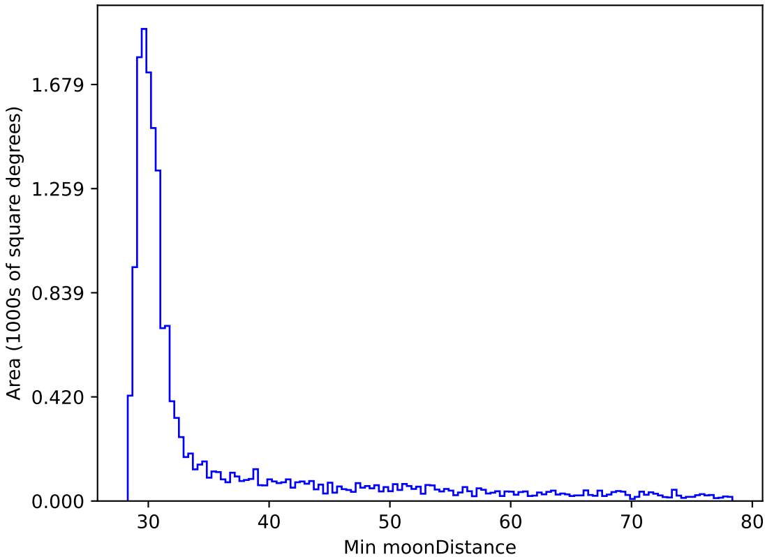
baseline_v3.2_10yrs WFD i band: Min moonDistance
