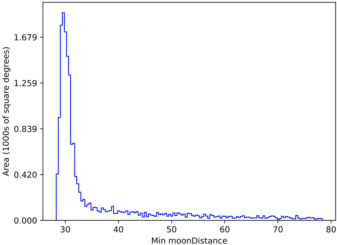
baseline_v3.2_10yrs WFD i band: Min moonDistance
