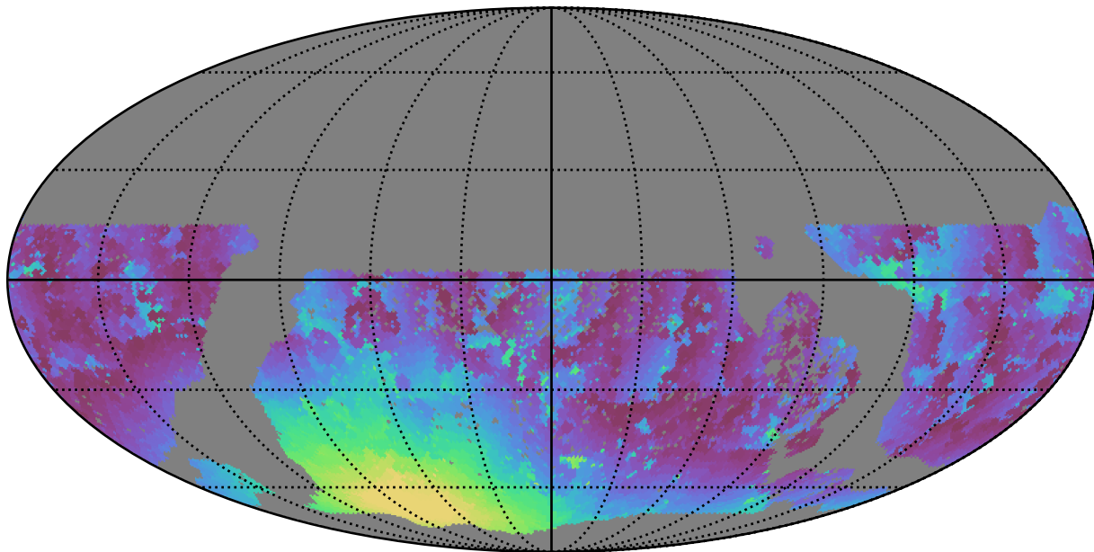
baseline_v3.2_10yrs WFD g band: Min moonDistance
