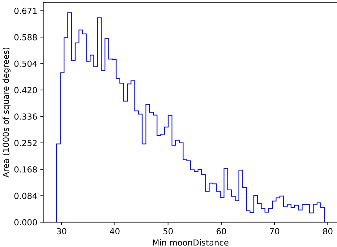
baseline_v3.2_10yrs WFD g band: Min moonDistance
