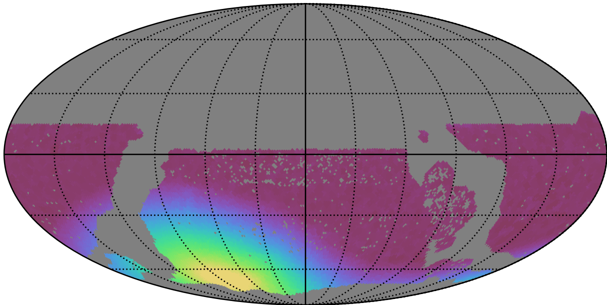
baseline_v3.2_10yrs WFD all bands: Min moonDistance
