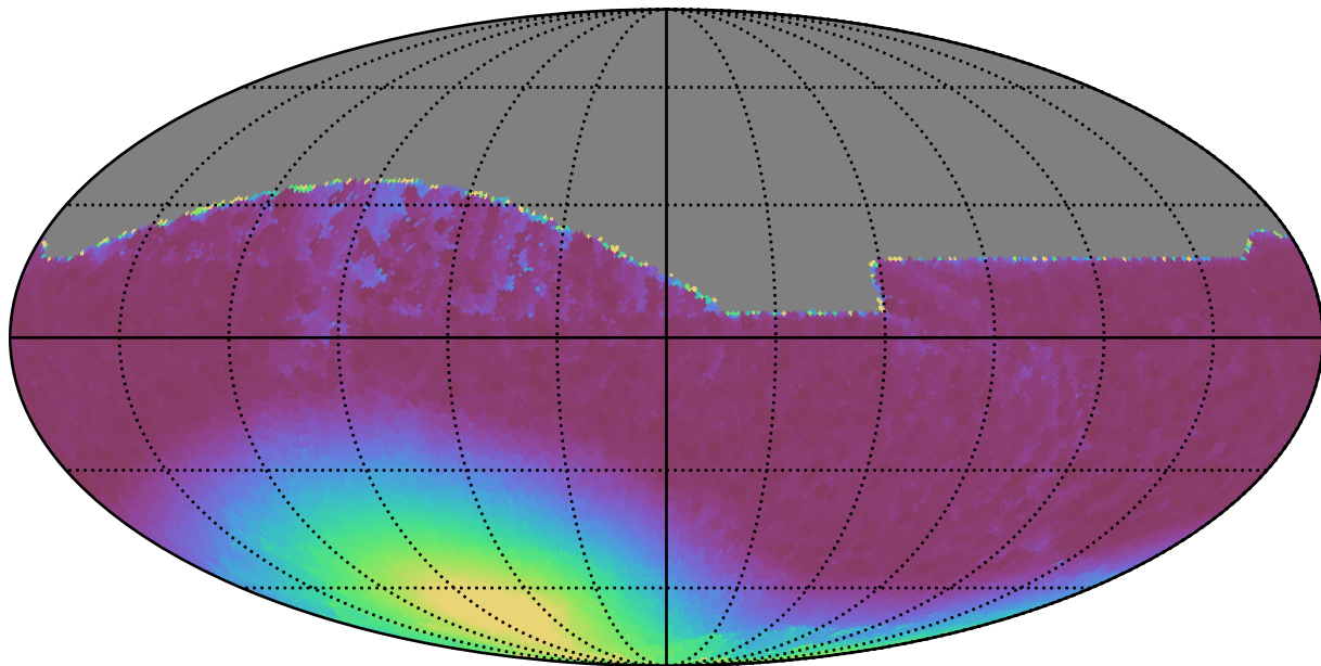
baseline_v3.2_10yrs All sky z band: Min moonDistance
