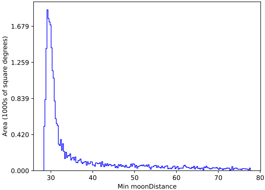
baseline_v3.2_10yrs All sky z band: Min moonDistance
