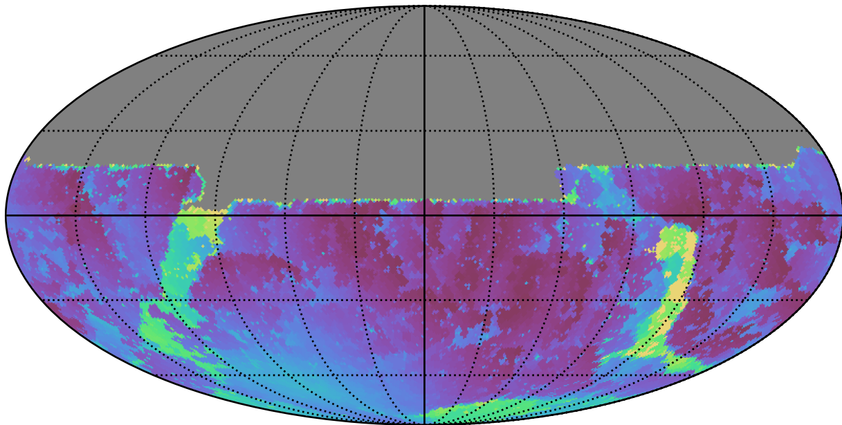
baseline_v3.2_10yrs All sky u band: Min moonDistance
