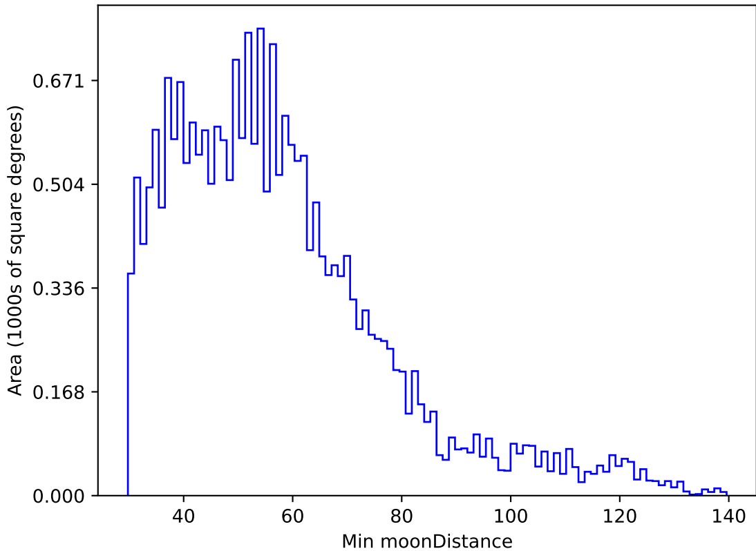
baseline_v3.2_10yrs All sky u band: Min moonDistance
