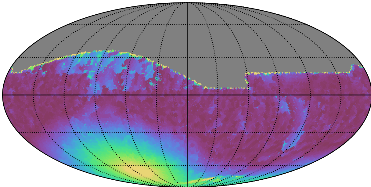
baseline_v3.2_10yrs All sky r band: Min moonDistance
