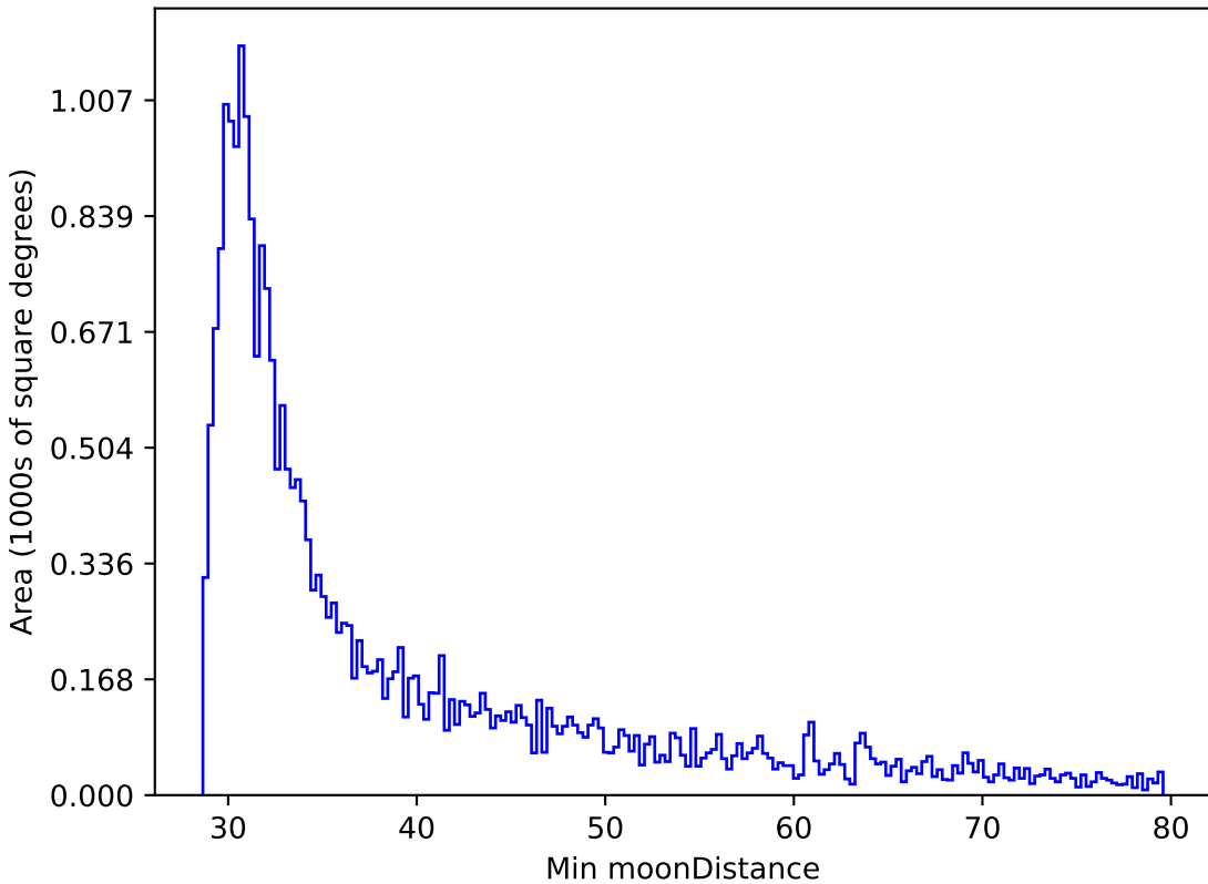
baseline_v3.2_10yrs All sky r band: Min moonDistance
