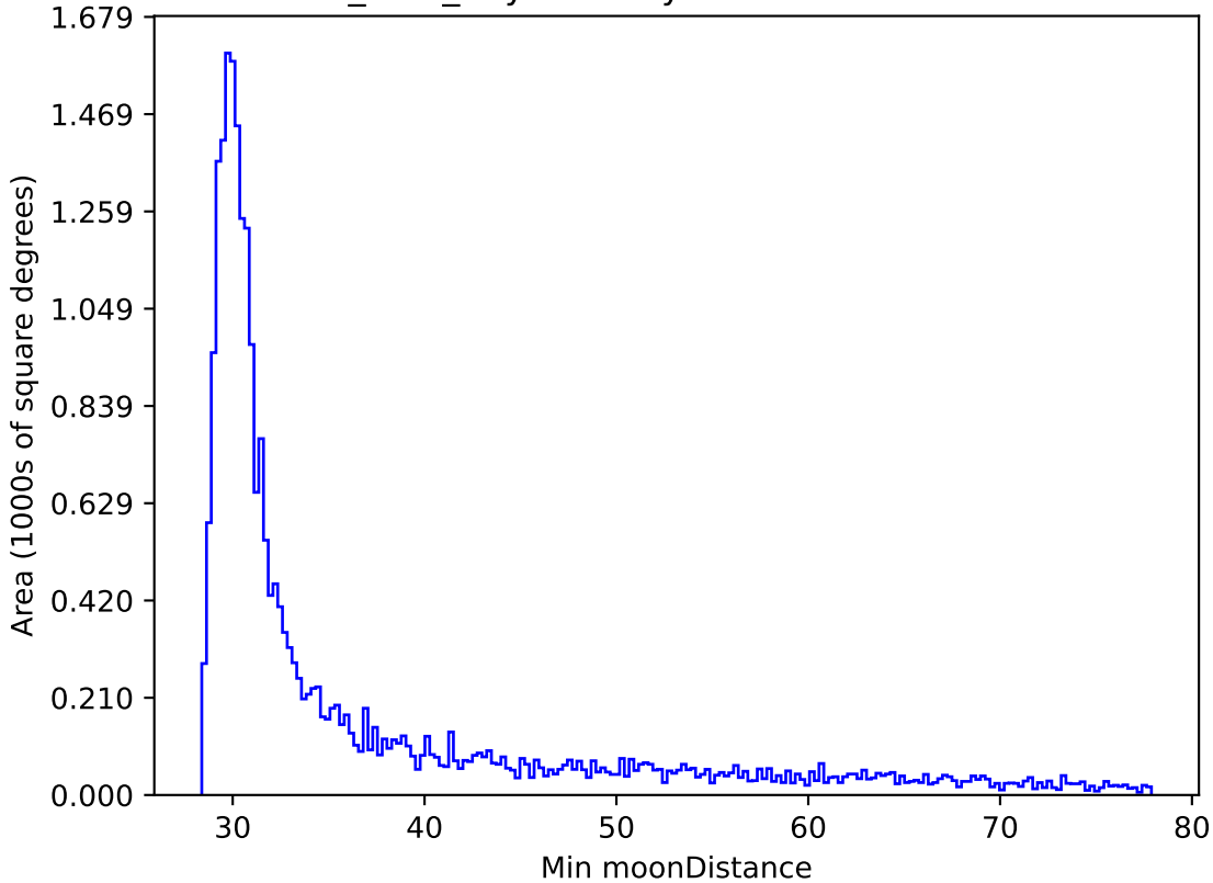
baseline_v3.2_10yrs All sky i band: Min moonDistance
