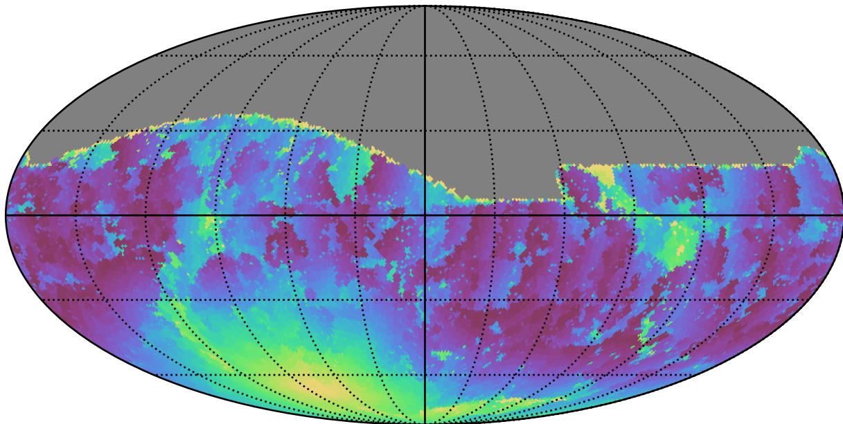
baseline_v3.2_10yrs All sky g band: Min moonDistance
