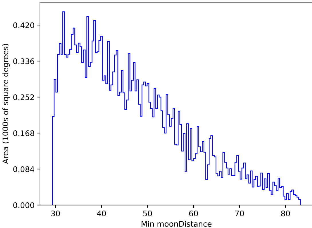
baseline_v3.2_10yrs All sky g band: Min moonDistance
