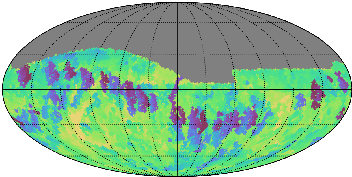
baseline_v3.2_10yrs Yr 1 z band: Min fiveSigmaDepth
