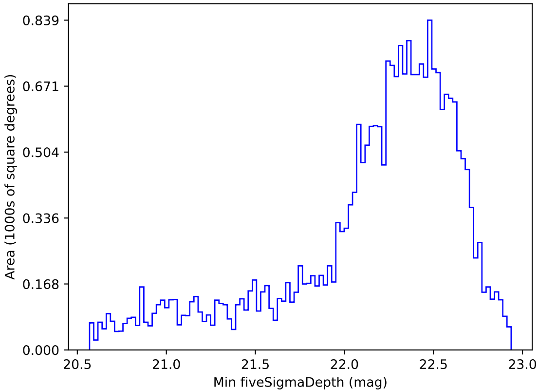
baseline_v3.2_10yrs Yr 1 z band: Min fiveSigmaDepth
