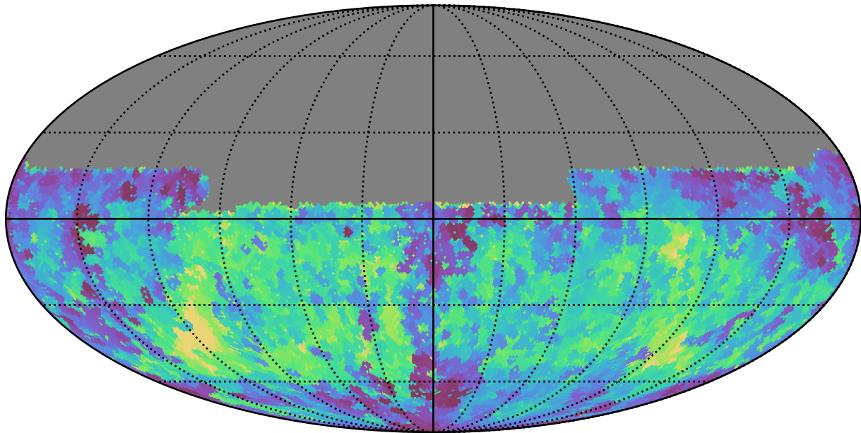
baseline_v3.2_10yrs Yr 1 y band: Min fiveSigmaDepth
