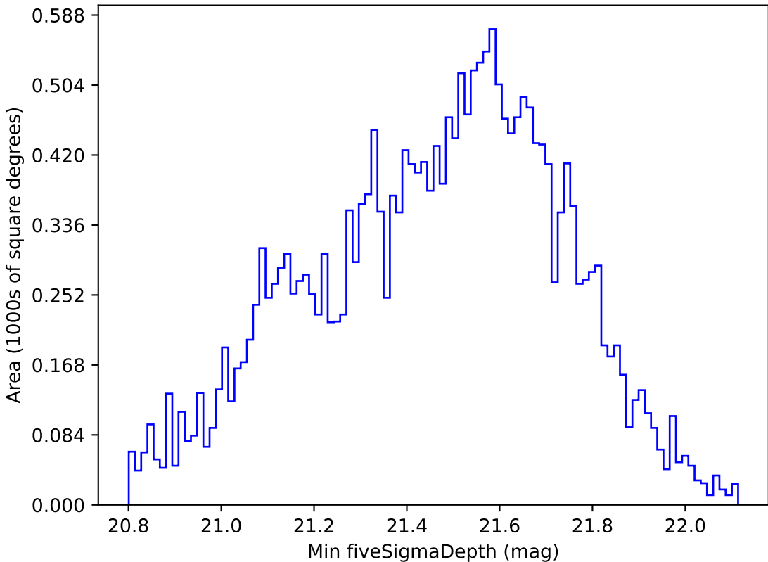
baseline_v3.2_10yrs Yr 1 y band: Min fiveSigmaDepth
