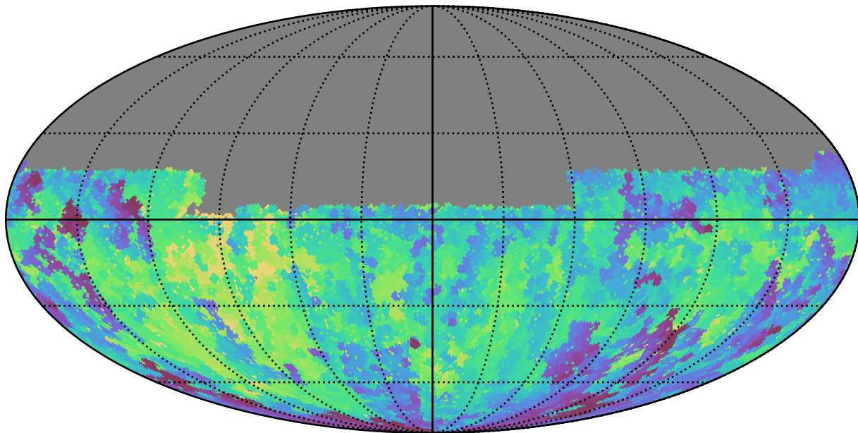
baseline_v3.2_10yrs Yr 1 u band: Min fiveSigmaDepth
