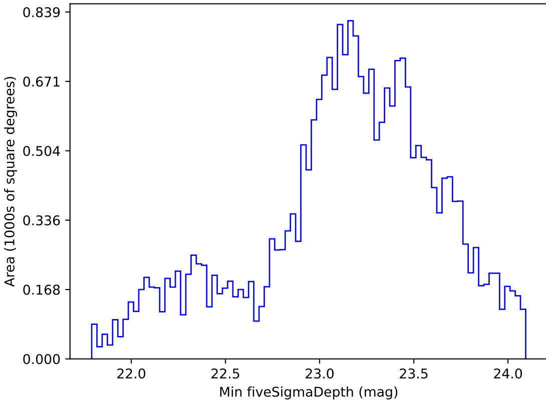
baseline_v3.2_10yrs Yr 1 r band: Min fiveSigmaDepth
