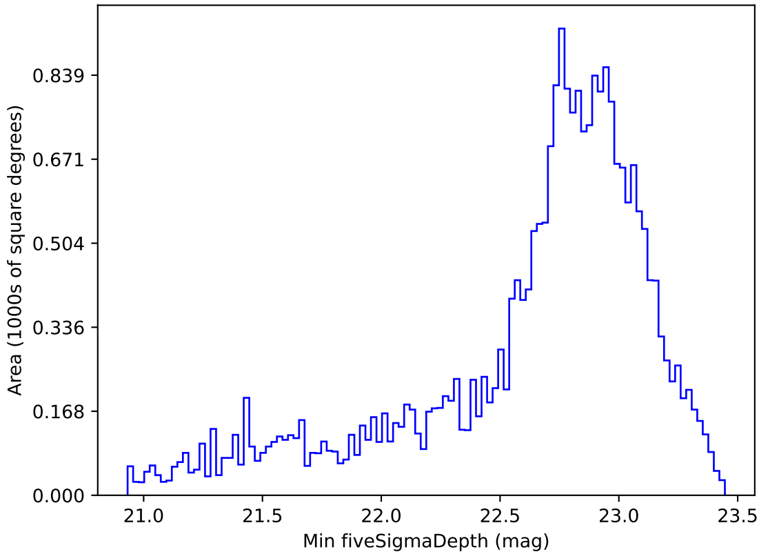
baseline_v3.2_10yrs Yr 1 i band: Min fiveSigmaDepth
