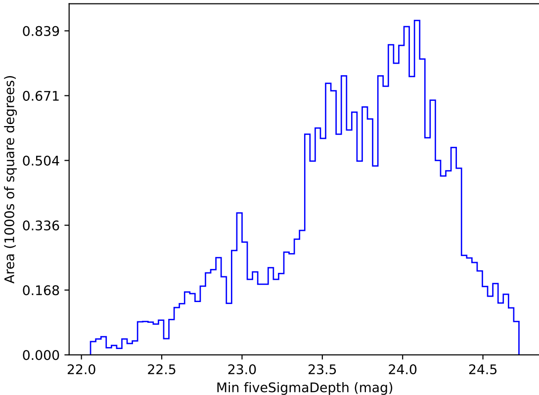
baseline_v3.2_10yrs Yr 1 g band: Min fiveSigmaDepth
