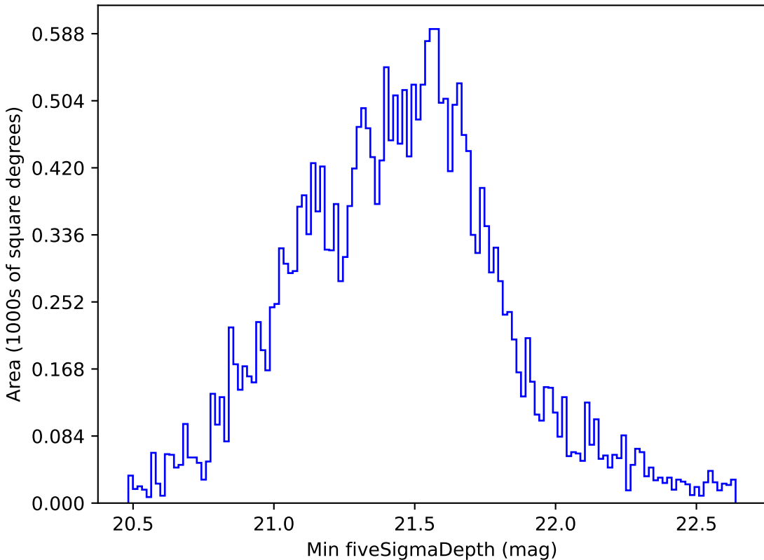
baseline_v3.2_10yrs Yr 1 all bands: Min fiveSigmaDepth
