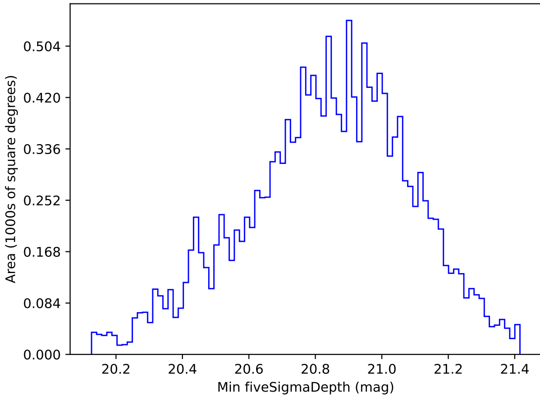
baseline_v3.2_10yrs WFD y band: Min fiveSigmaDepth
