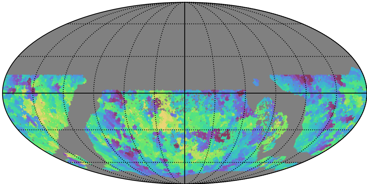
baseline_v3.2_10yrs WFD u band: Min fiveSigmaDepth
