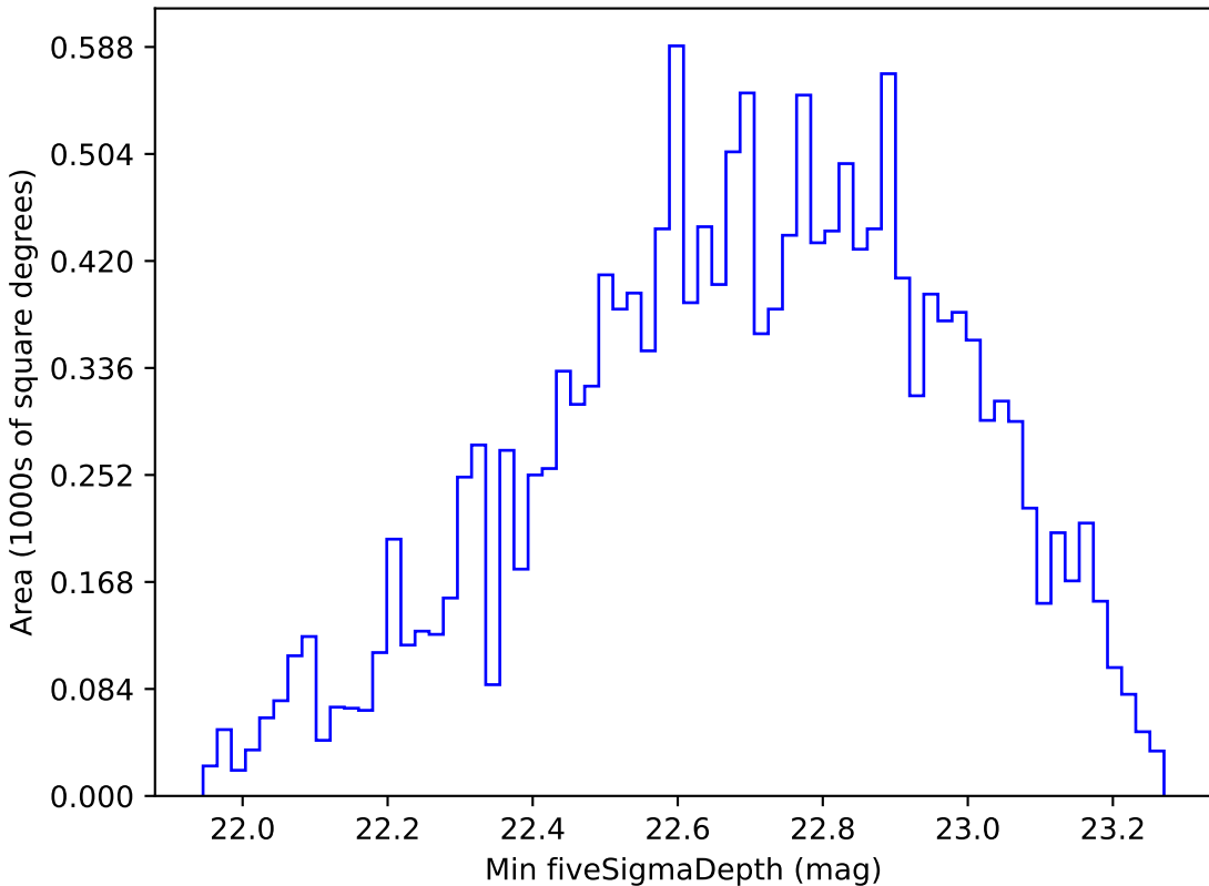
baseline_v3.2_10yrs WFD u band: Min fiveSigmaDepth
