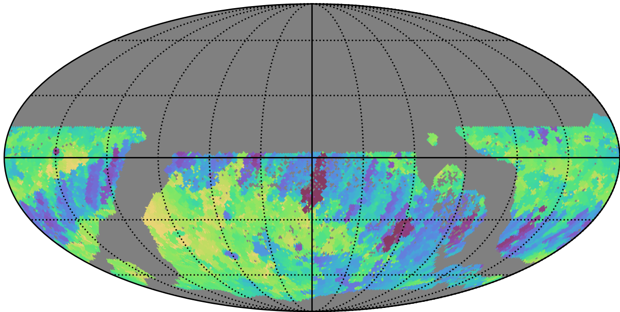
baseline_v3.2_10yrs WFD r band: Min fiveSigmaDepth
