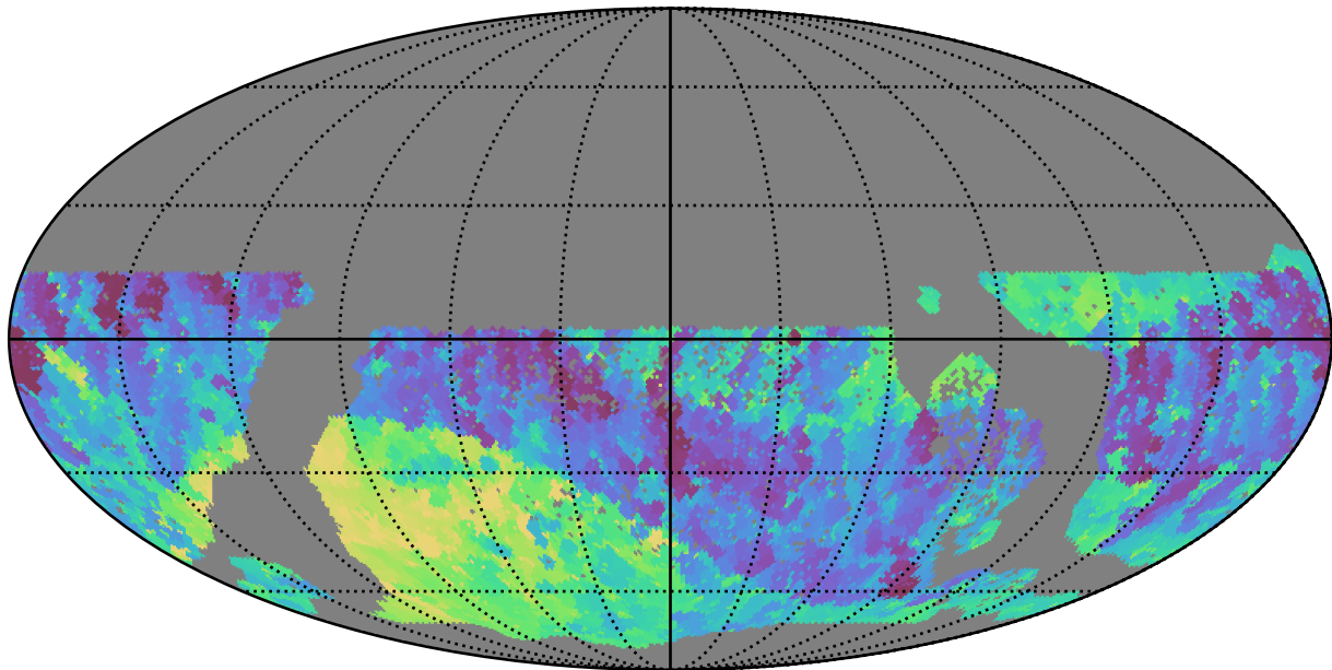
baseline_v3.2_10yrs WFD i band: Min fiveSigmaDepth
