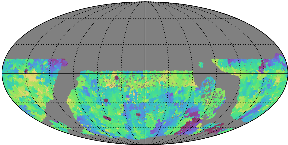
baseline_v3.2_10yrs WFD g band: Min fiveSigmaDepth
