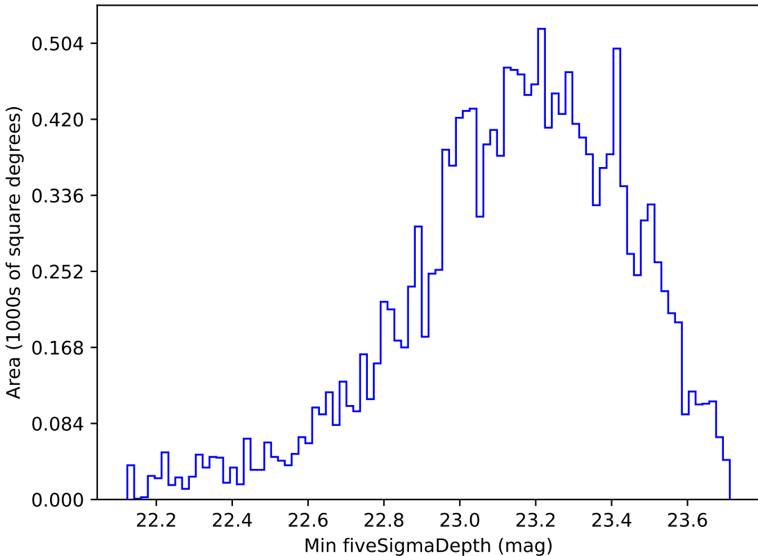
baseline_v3.2_10yrs WFD g band: Min fiveSigmaDepth
