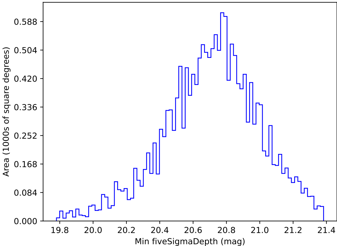
baseline_v3.2_10yrs WFD all bands: Min fiveSigmaDepth
