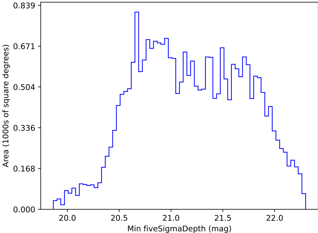
baseline_v3.2_10yrs All sky z band: Min fiveSigmaDepth
