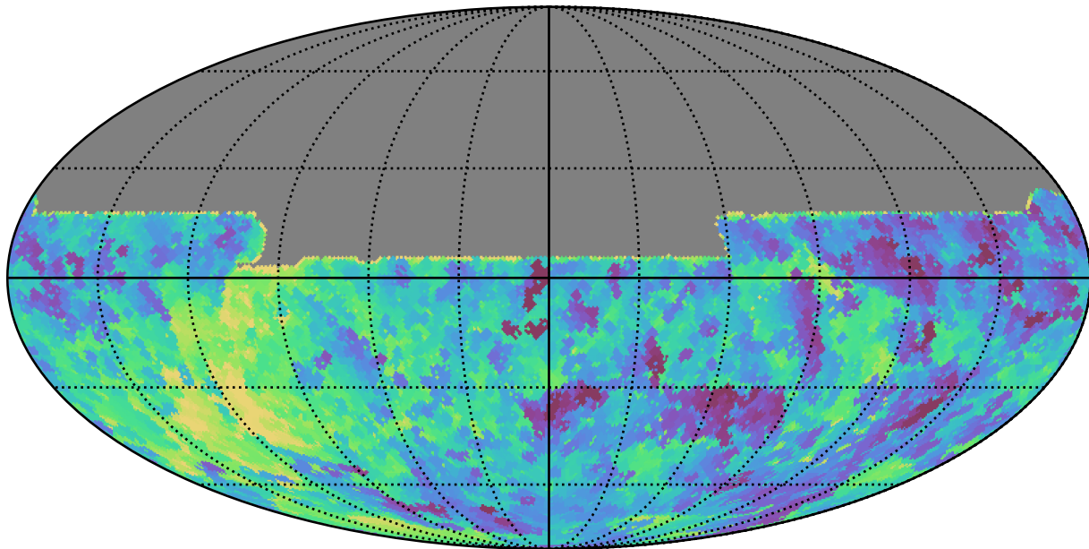
baseline_v3.2_10yrs All sky y band: Min fiveSigmaDepth
