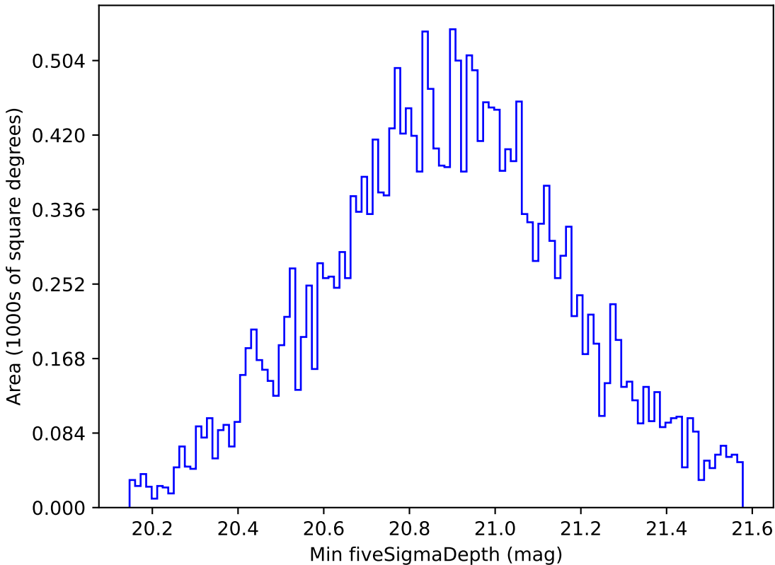
baseline_v3.2_10yrs All sky y band: Min fiveSigmaDepth
