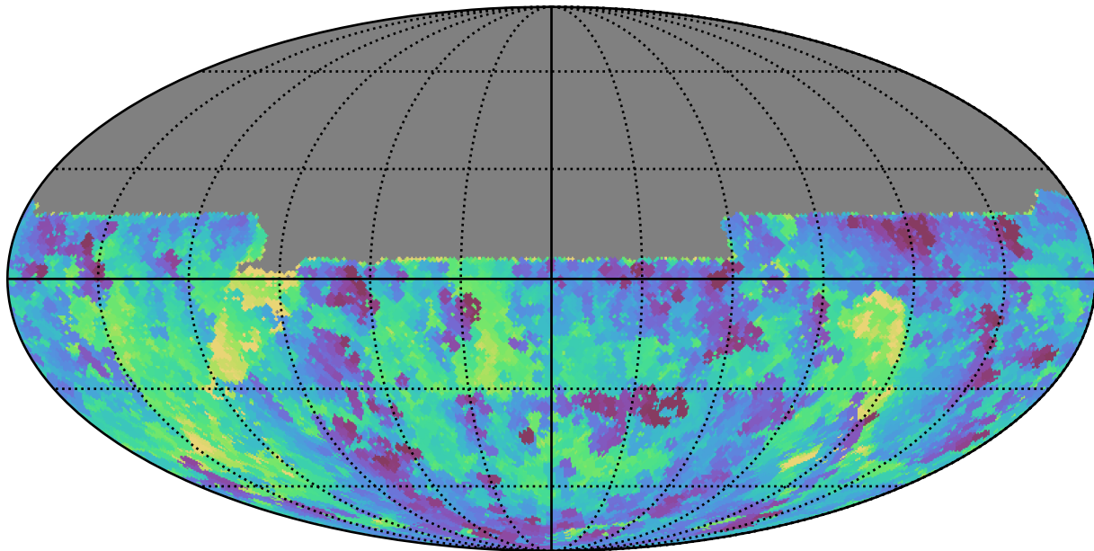
baseline_v3.2_10yrs All sky u band: Min fiveSigmaDepth
