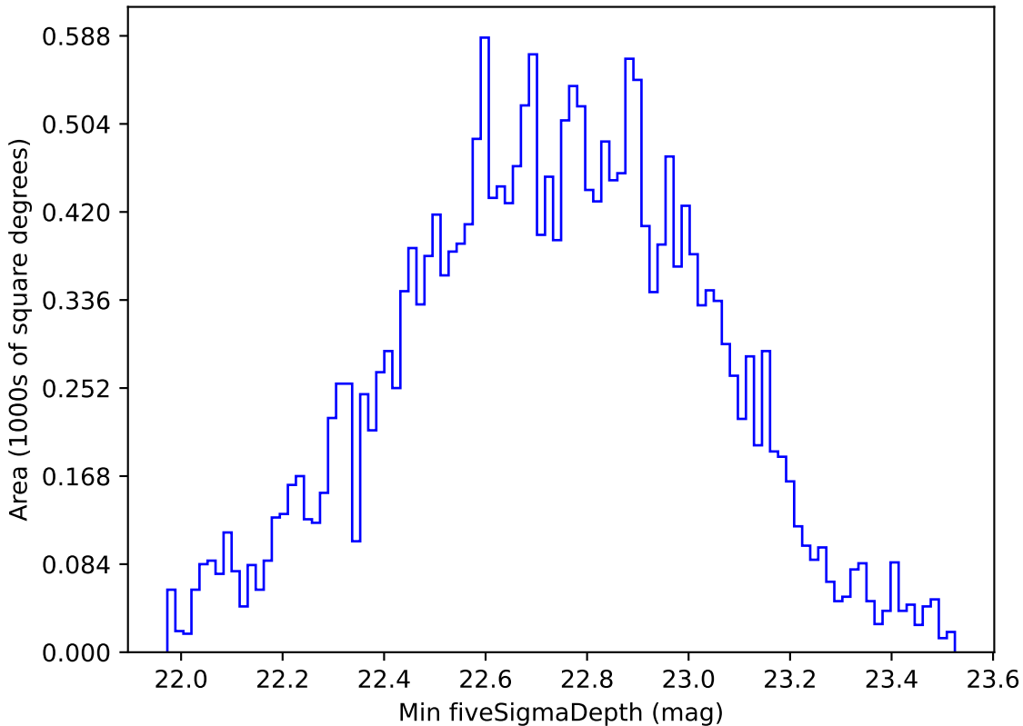
baseline_v3.2_10yrs All sky u band: Min fiveSigmaDepth
