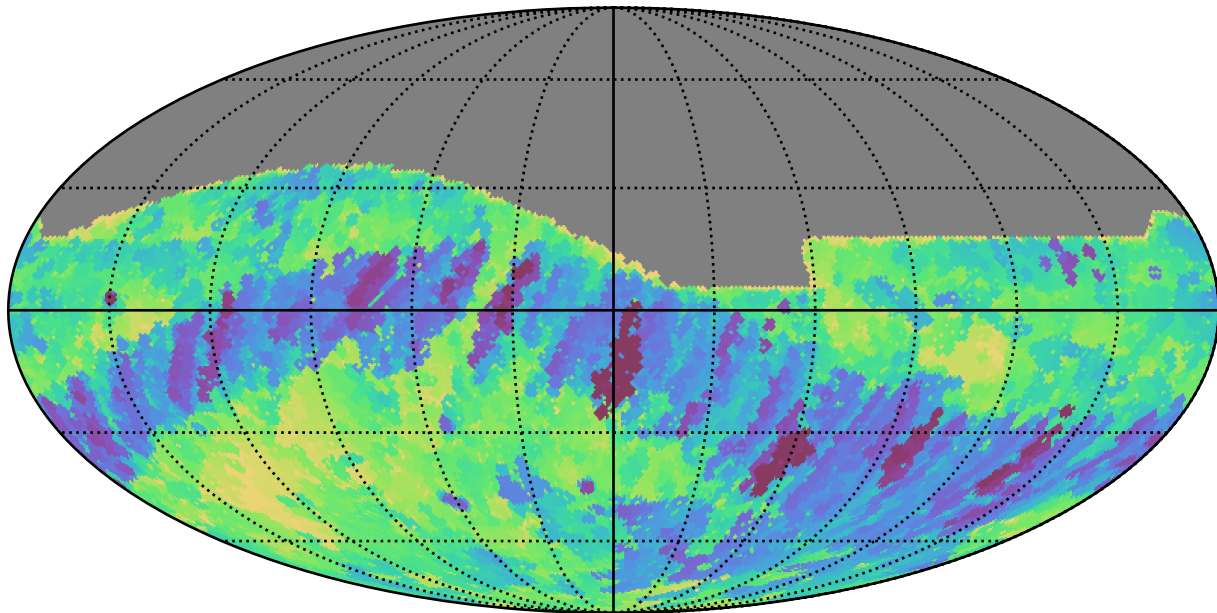
baseline_v3.2_10yrs All sky r band: Min fiveSigmaDepth
