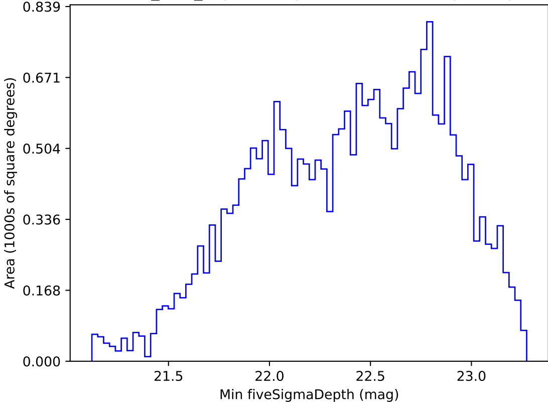
baseline_v3.2_10yrs All sky r band: Min fiveSigmaDepth
